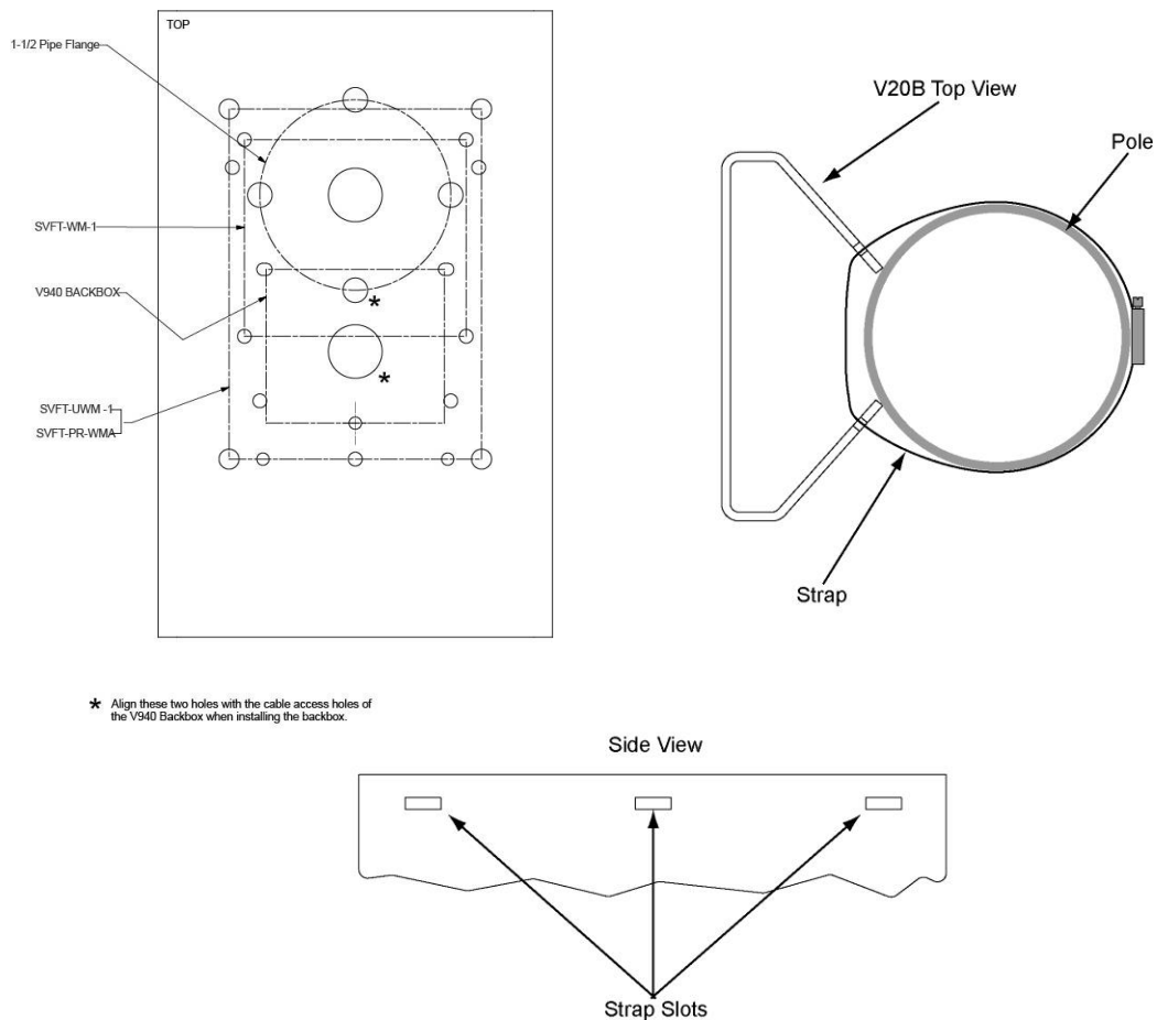
Figure 1 Pole Mounting Adapter Installation
